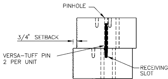
Pinning Detail
