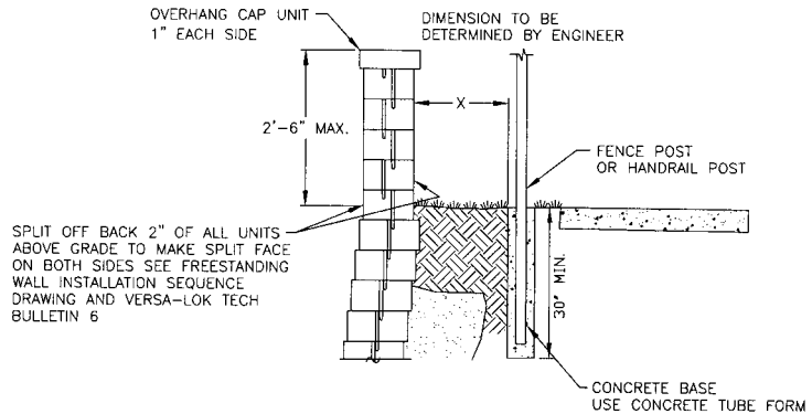
FREESTANDING WALL DETAIL (STRAIGHT WALLS ONLY) TYPICAL HANDRAIL AND/OR FENCE POST SCALE: 1/2"=1'
