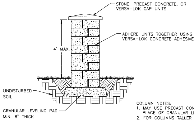
COLUMN SECTION UNREINFORCED COLUMN (4' TALL MAX.) SCALE: 3/4"=1'
