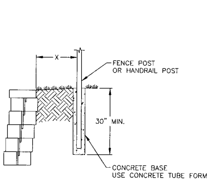
POST DETAIL TYPICAL HANDRAIL AND/OR FENCE POST SCALE: NONE
